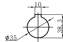
细节A 5:1 (DETAIL A 5:1)
